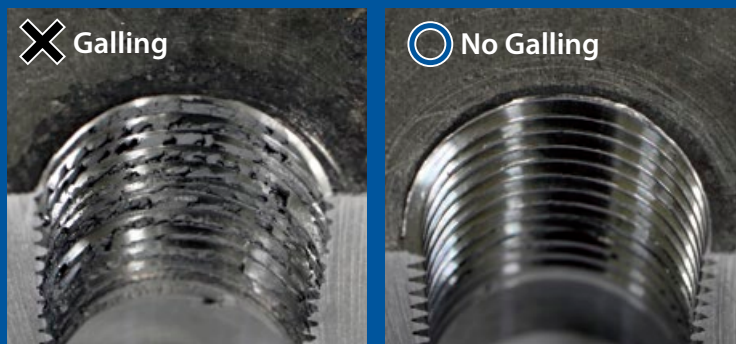
SS400材での加工イメージ Image to process taper pipe thread in SS400 material
